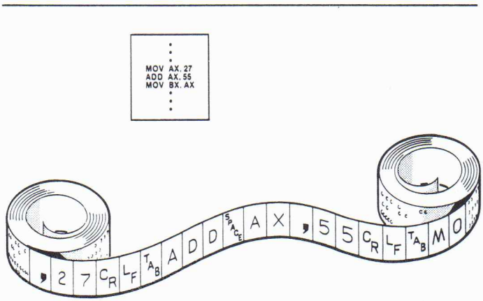
Figure 7-1. Macro Processor versus Assembler — Two Different Views of a Source File
