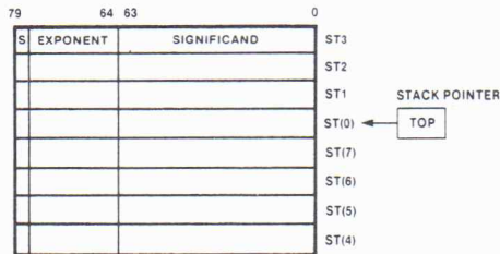
Figure 6-1. The 8087 Stack Fields
