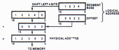
Figure 1-4. Generating a Physical Address
