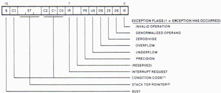
Figure 6-3. Status Word Format
