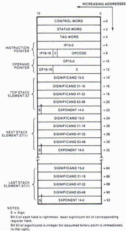
Figure 6-8. FSAVE/FRSTOR Memory Layout
