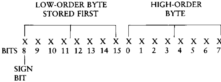
Figure 6-3. Integer Storage
