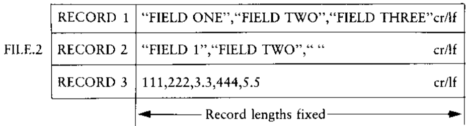
Figure 5-2. Relative File
