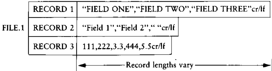
Figure 5-1. Sequential File
